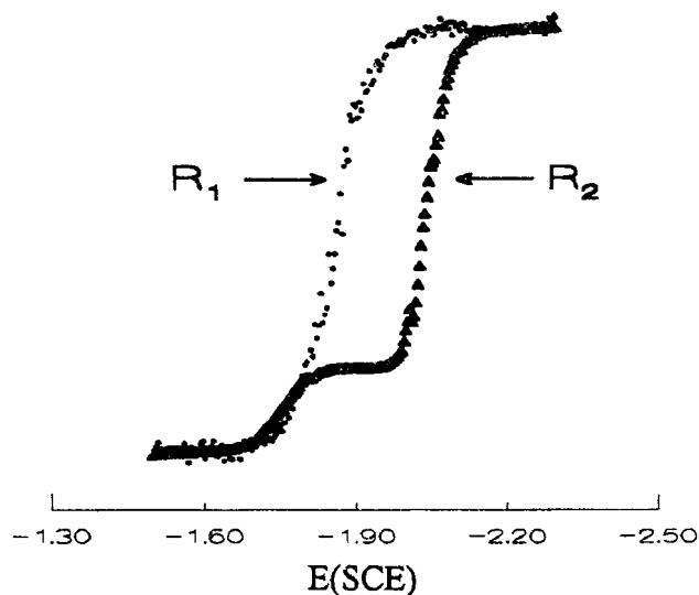
Fig. 2. Steady-state voltammogram of \text{Cp}(\text{CO})_2\text{Fe}(\text{COCH}_2\text{CH}_2\text{Ph}) , 2 mM solution in THF/0.3 M \text{Bu}_4\text{BF}_4 at a gold electrode (25 \mu\text{m} diameter); potential scan rate 10 \text{ mV s}^{-1} . ●, complex alone; ▲, in the presence of 5 molar equivalents of \text{Bu}_3\text{SnH} .
